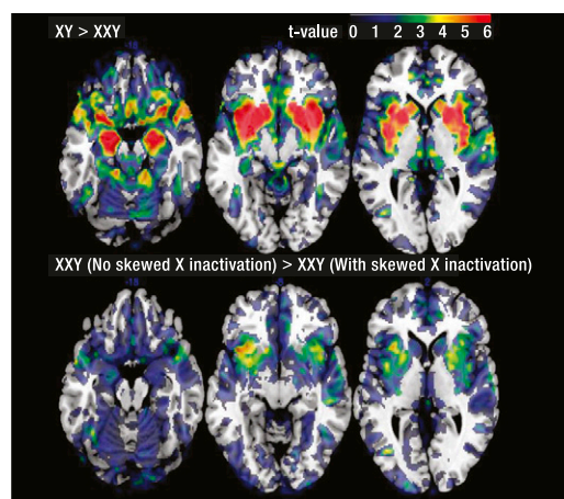
Figure 6. Bilateral ventral and subcortical gray matter volume in brain areas in KS. Bilateral ventral and subcortical gray matter volume in brain areas, including hippocampus, insula, and striatum, is found to be smaller in KS males relative to 46,XY males. A subset of KS males has skewed X chromosome inactivation. This group shows an exacerbated pattern of decreased regional gray matter volume. Figure shows unthresholded t maps for display purposes. Includes data from Skakkebaek et al. (73, 256).
